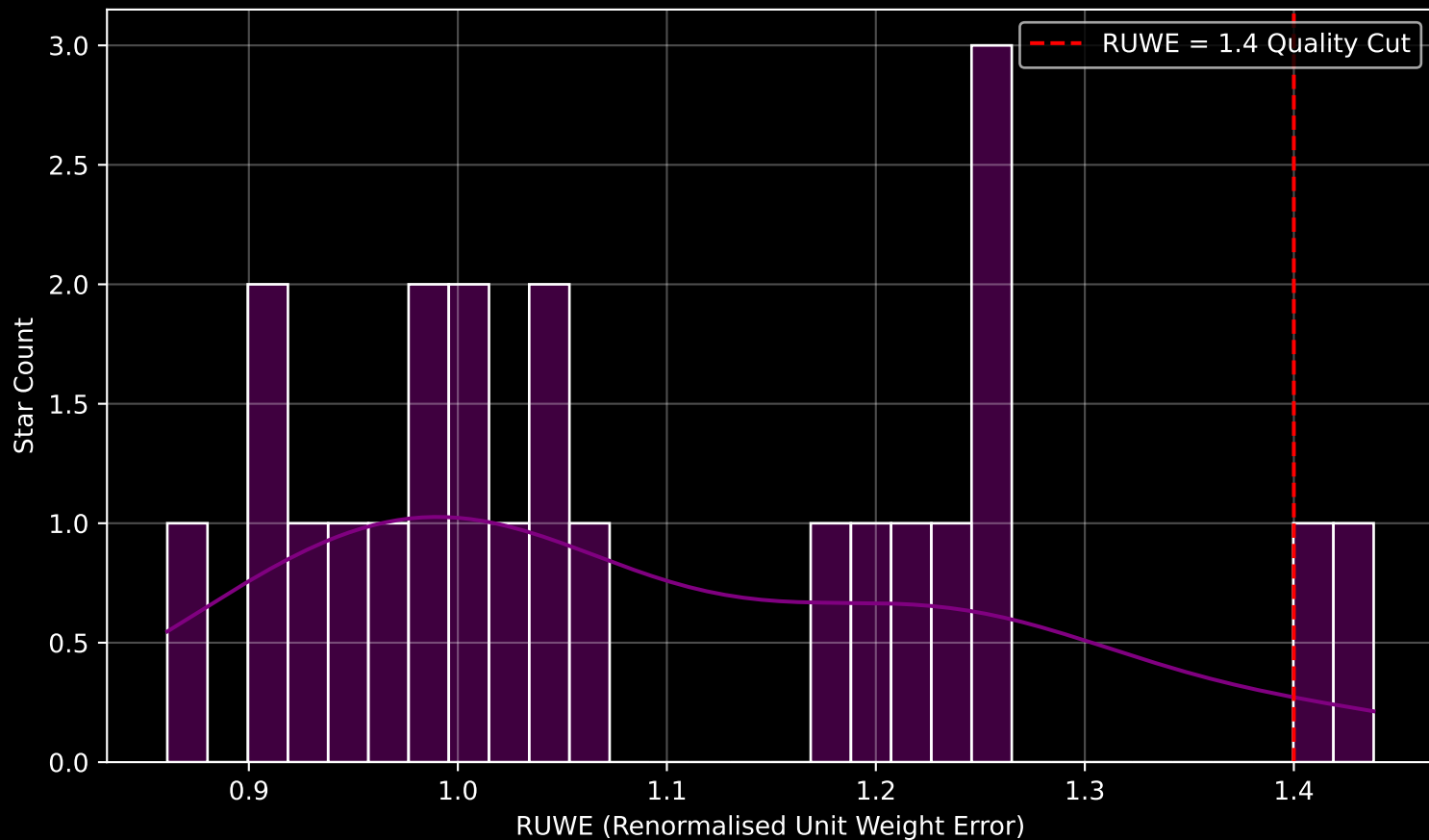
GAPOGEE DR17 Field [rrlyr] RUWE Distribution (n= 23)
