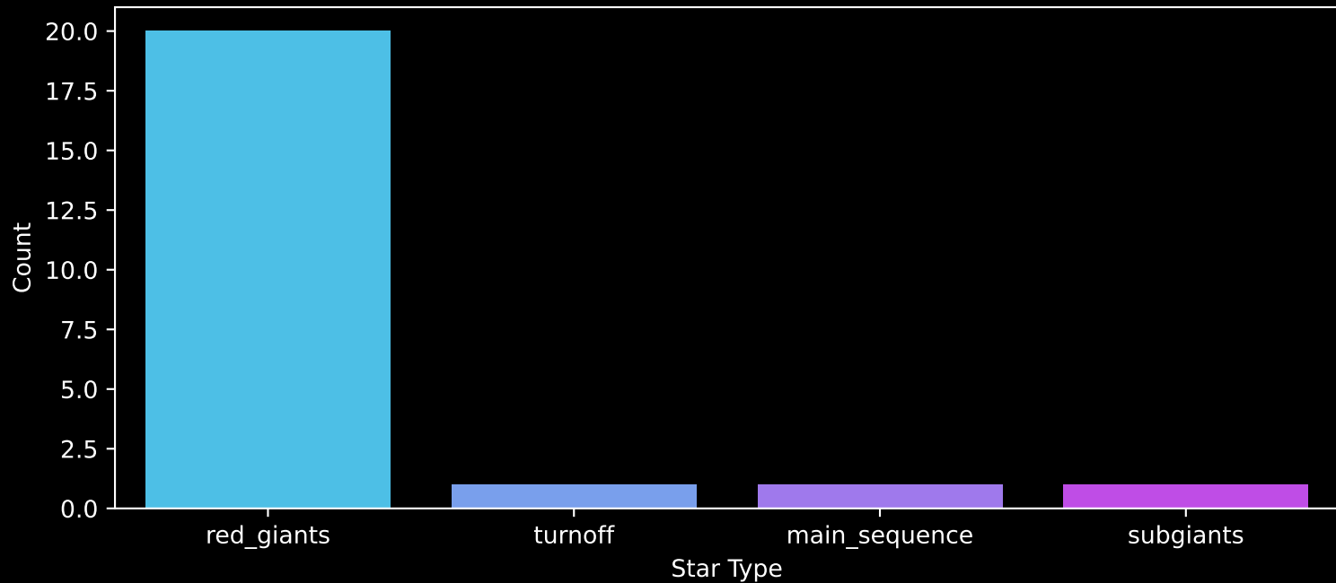
APOGEE DR17 Field: [rrlyr] Count plot of Star Type
