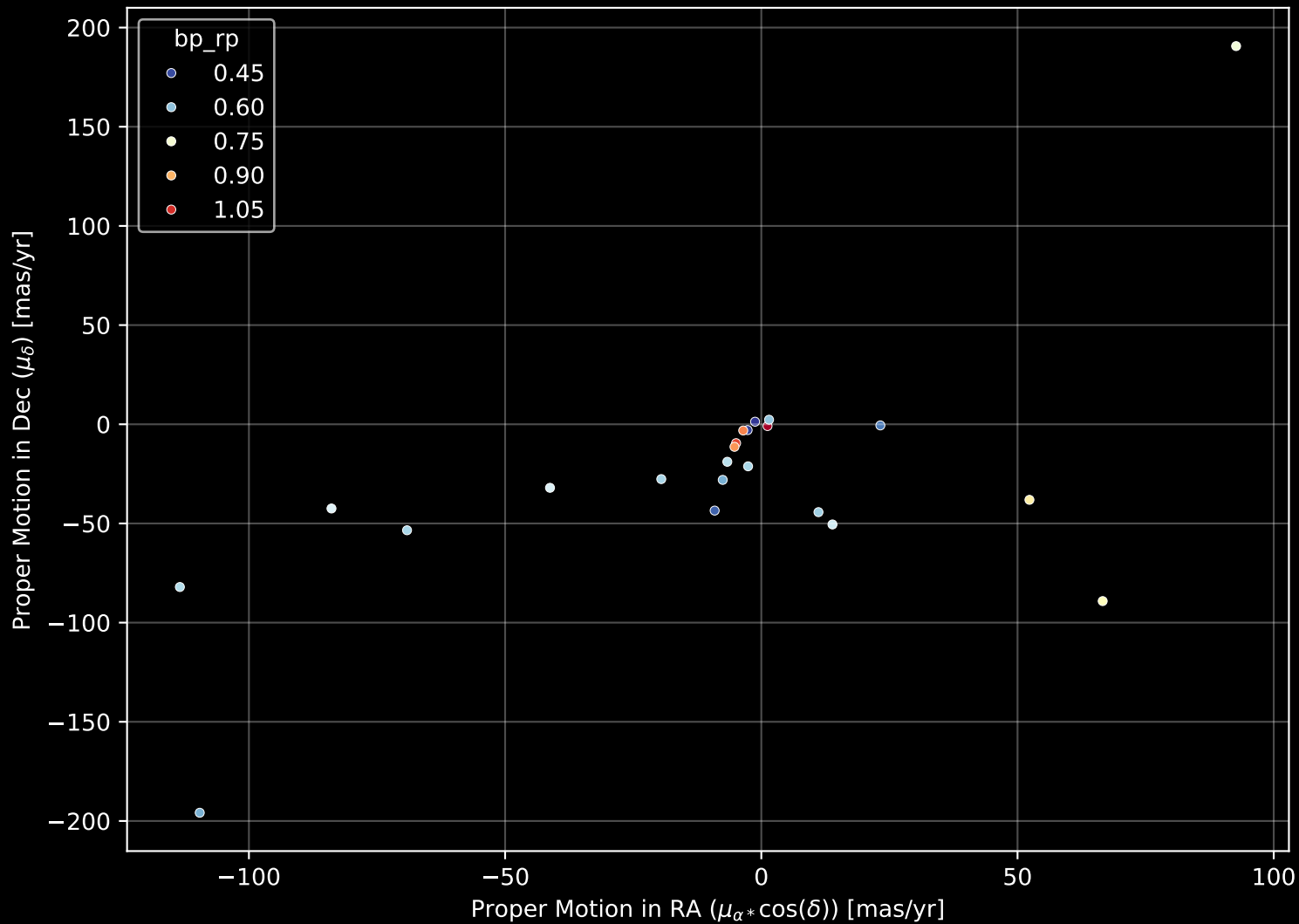
APOGEE DR17 Field: [rrlyr] Proper Motion Diagram (n= 23)
