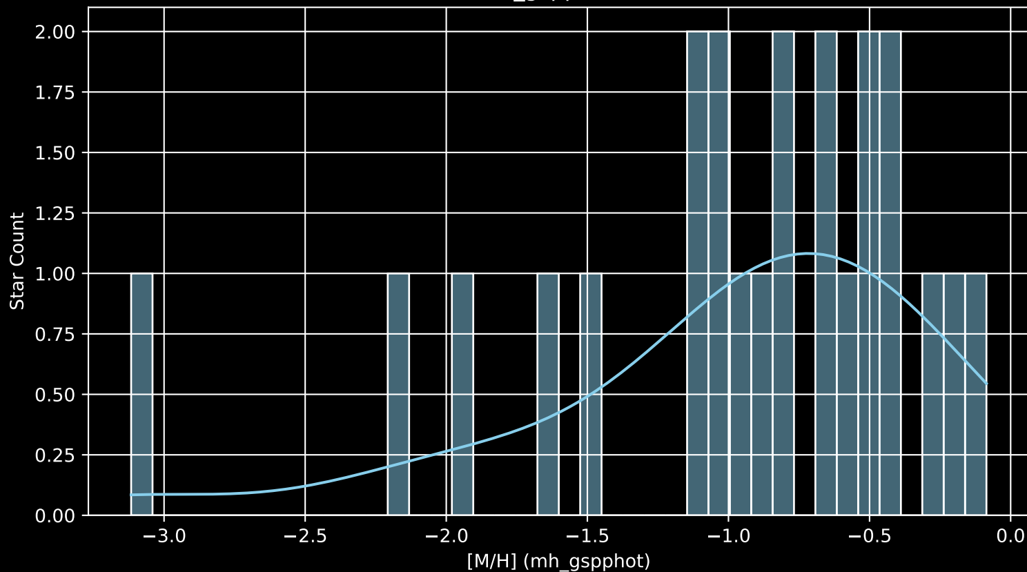
APOGEE DR17 Field: [rrlyr [M/H] (mh_gspphot) (n= 23)
