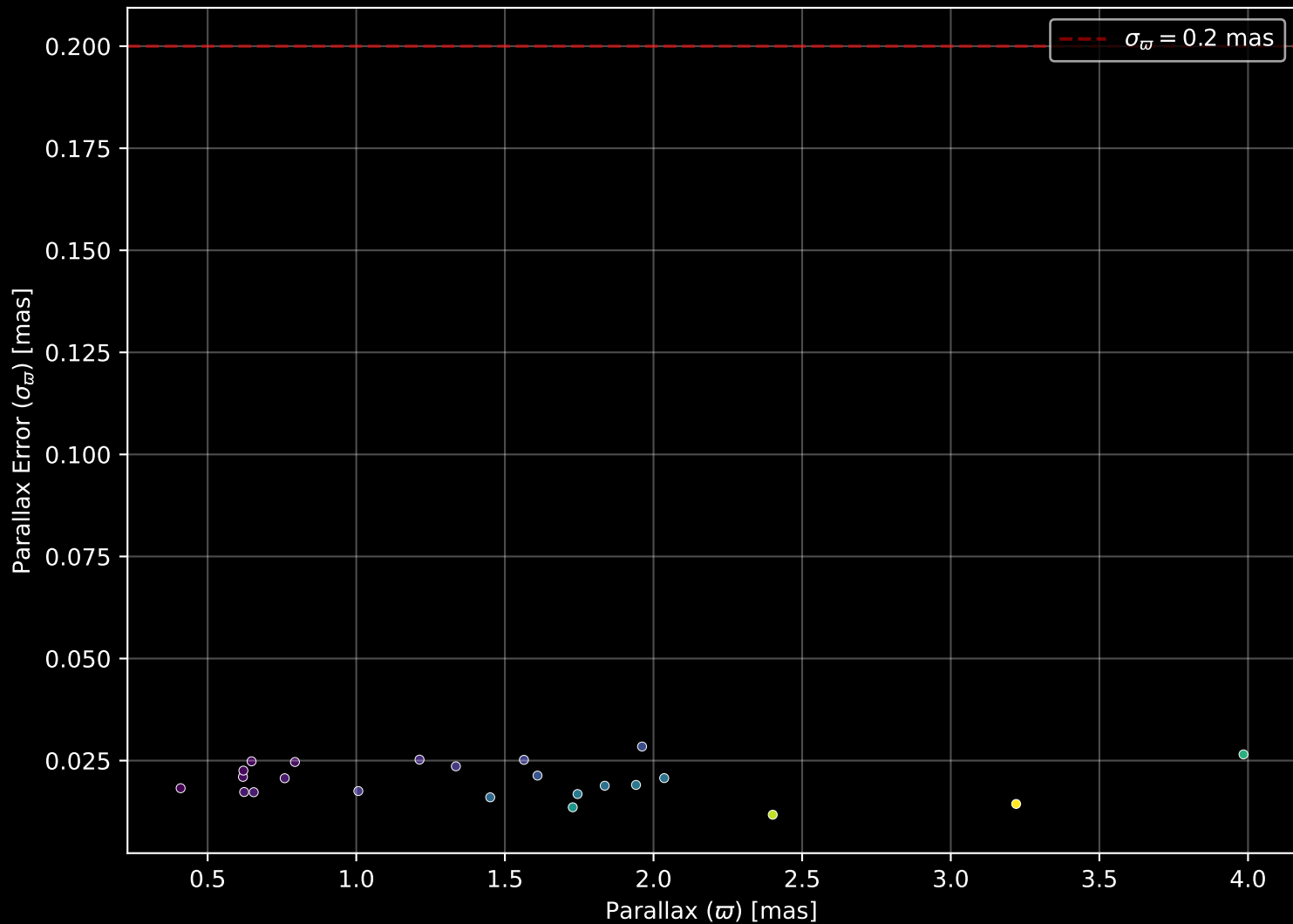
APOGEE DR17 Field: [rrlyr] Parallax Quality (n= 23)
