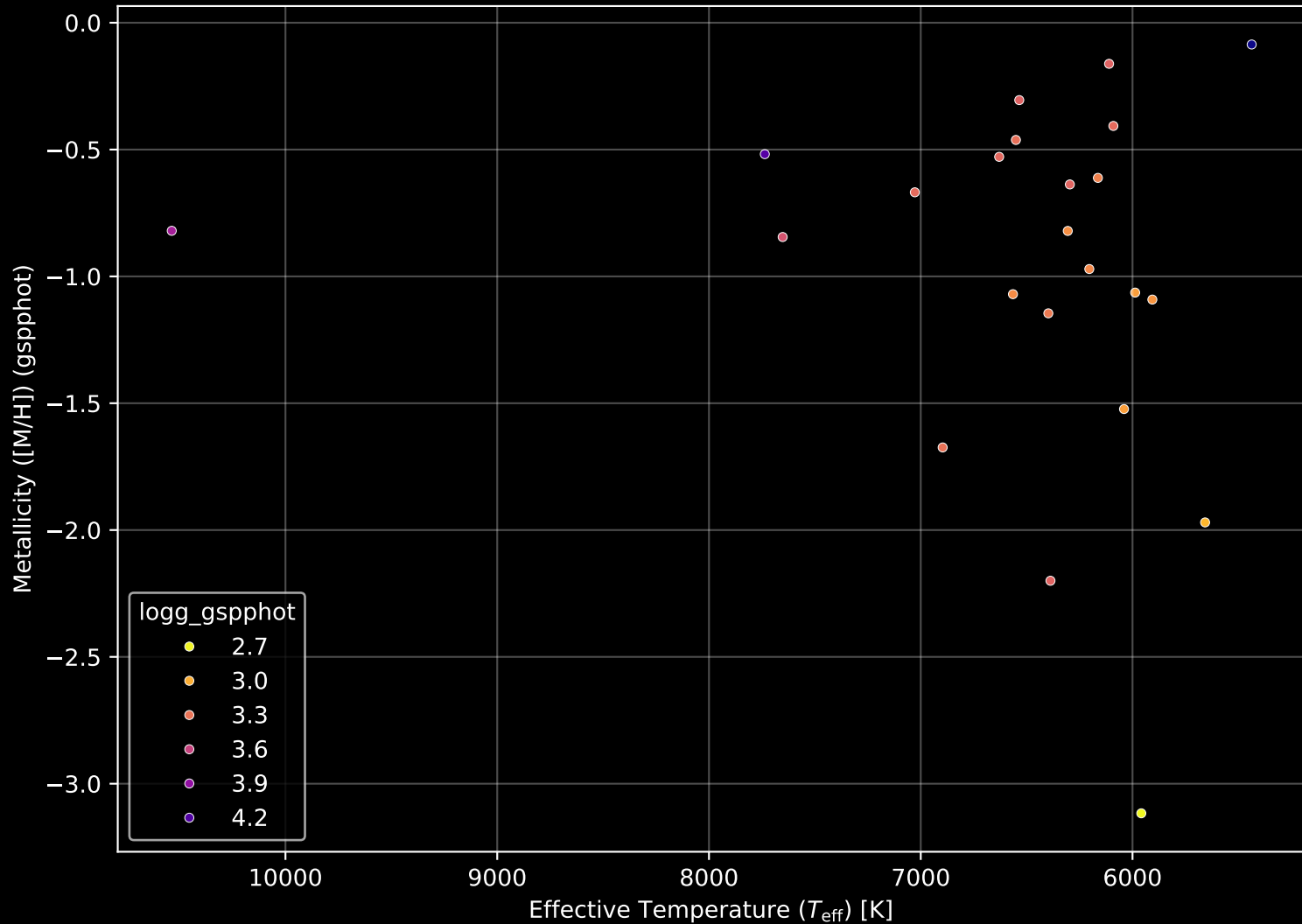
APOGEE DR17 Field: [rrlyr] Stellar Population Parameters (n= 23)
